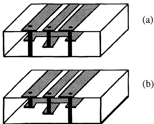
Figure 6. Two possible interconnect techniques for the CBCPW to 3-wire line to stripline transition.
