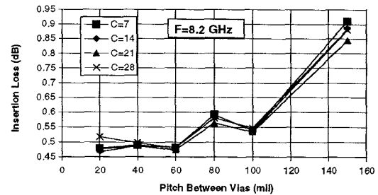
Figure 3. Insertion loss as a function of via pitch and distance from the inside edge of the topside grounds.
