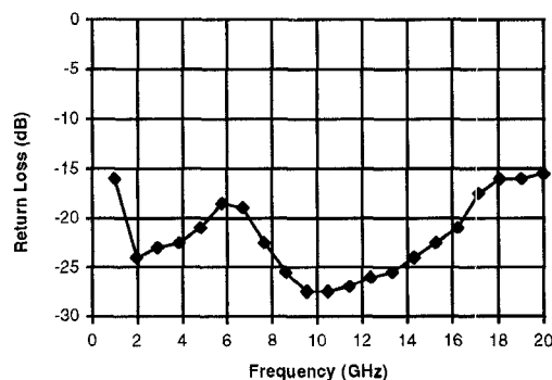
Figure 7. Measured performance of the CBCPW to 3-wire line to button connector.
