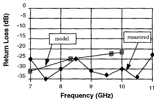
Figure 9. Measured and modeled performance of the CBCPW to microstrip transition. Transition length = 150 mil.
