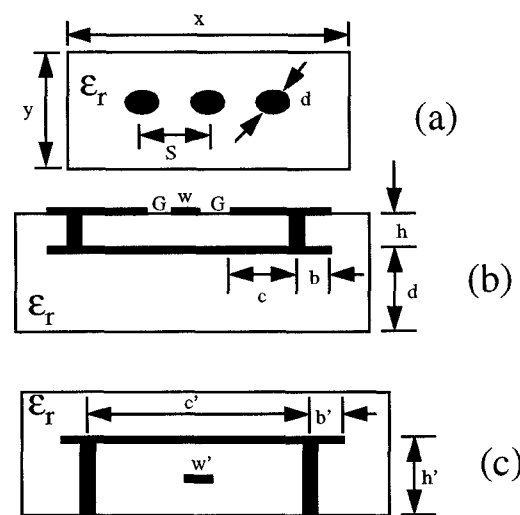
Figure 1. Transmission Lines Used.
