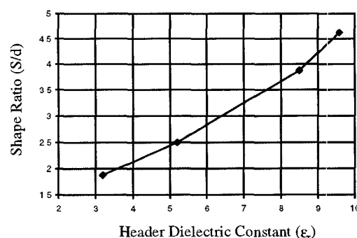
Figure 2. Finite element modeling of the required shape ratio to obtain a 50 ohm 3-wire line for various header dielectric constants.
