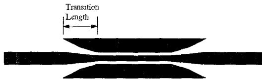
Figure 8. Illustration of the microstrip to CBCPW transition.
