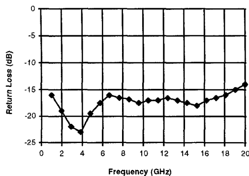
Figure 5. Measured performance of the CBCPW to 3-wire line transition.
