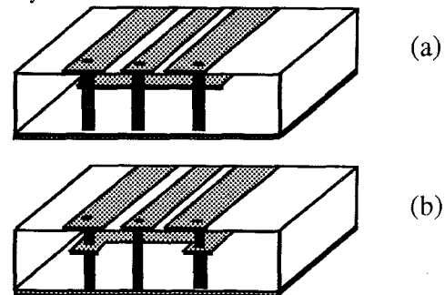
Figure 4. Two approaches for CBCPW to 3-wire line transition.
